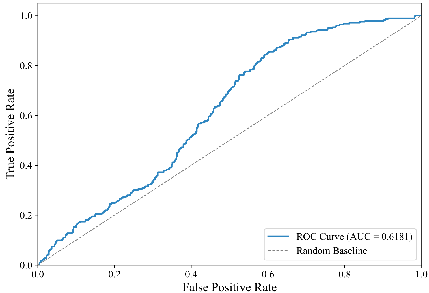
ROC Curve — ENGLISH_MANUAL (xlm-roberta-base, lightgbm)
