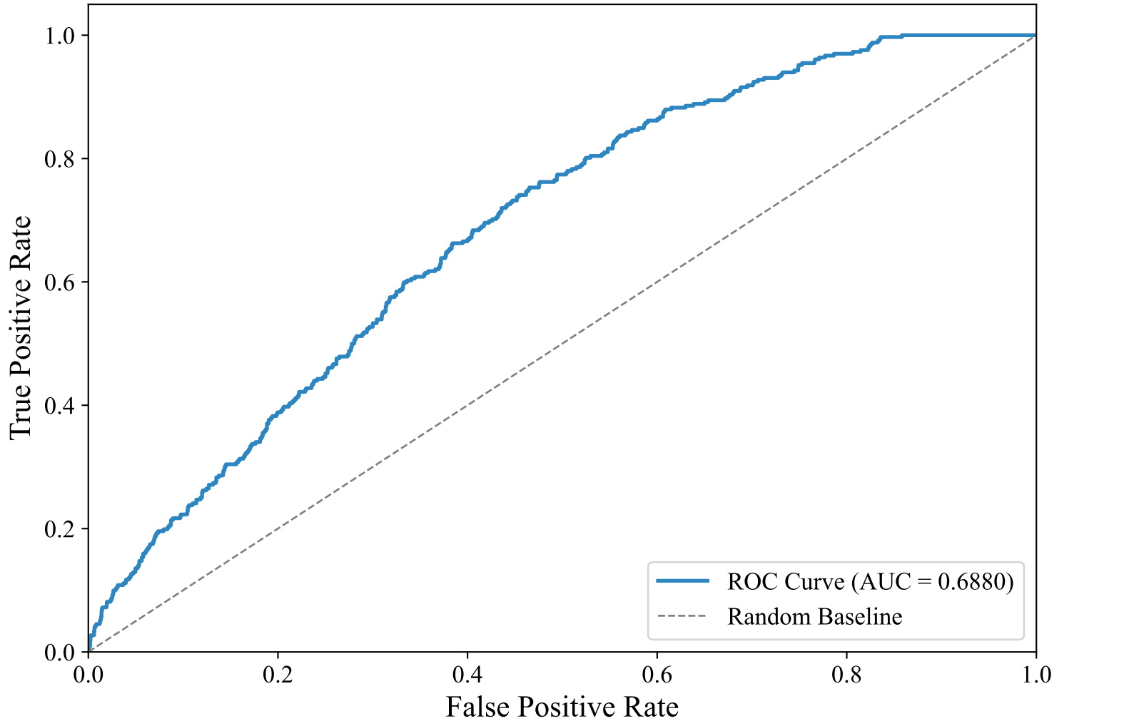
ROC Curve — GERMAN_MANUAL (bert-base-multilingual-uncased, svm_linear)
