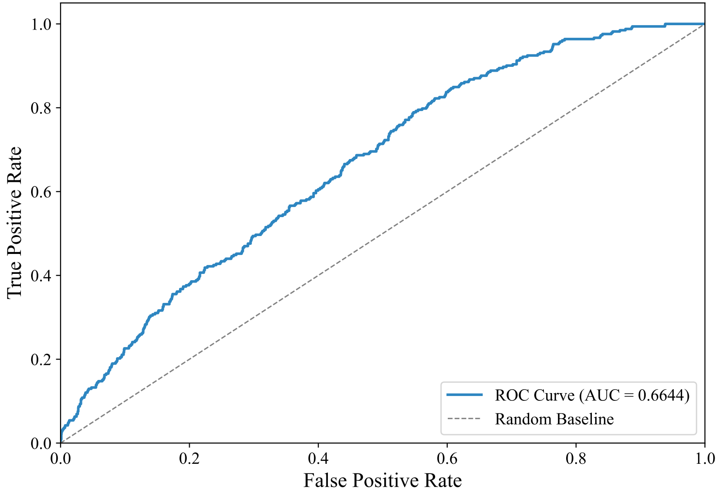
ROC Curve — GERMAN_MANUAL (multilingual-e5-large-instruct, random_forest)
