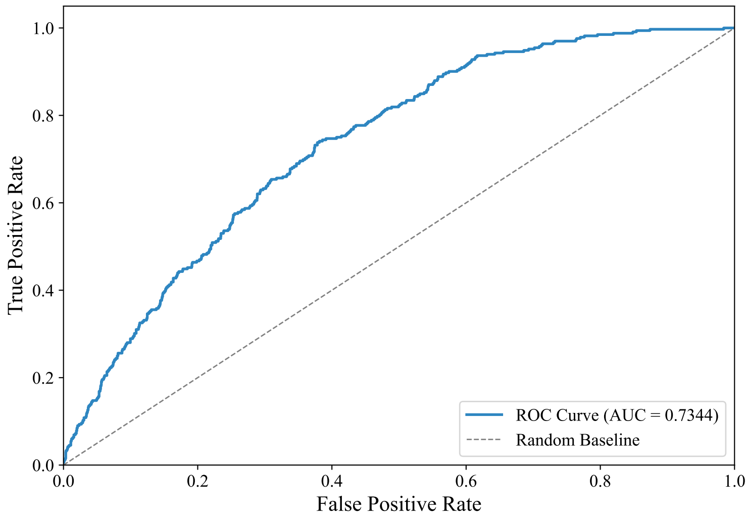
ROC Curve — GERMAN_MANUAL (multilingual-e5-large-instruct, svm_linear)
