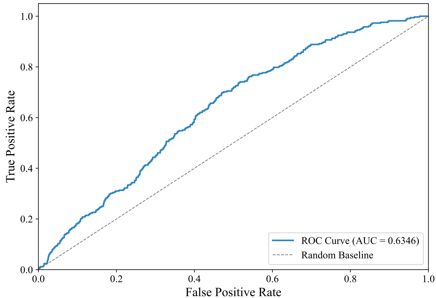
ROC Curve — GERMAN_MANUAL (paraphrase-multilingual-MiniLM-L12-v2, xgboost)
