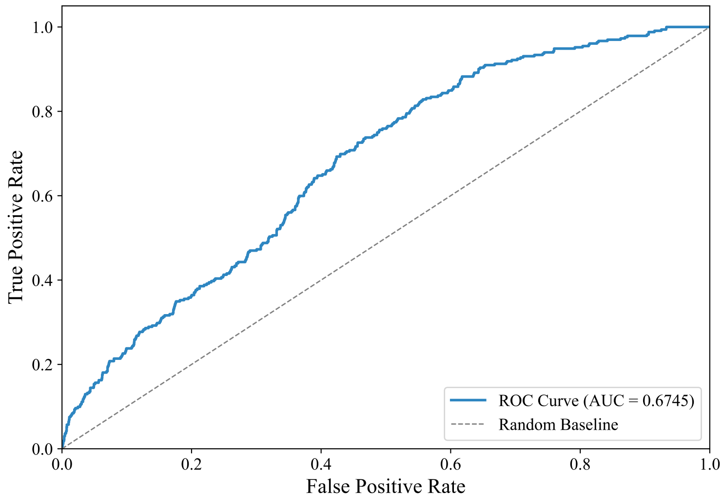
ROC Curve — GERMAN_MANUAL (paraphrase-multilingual-mpnet-base-v2, svm_linear)
