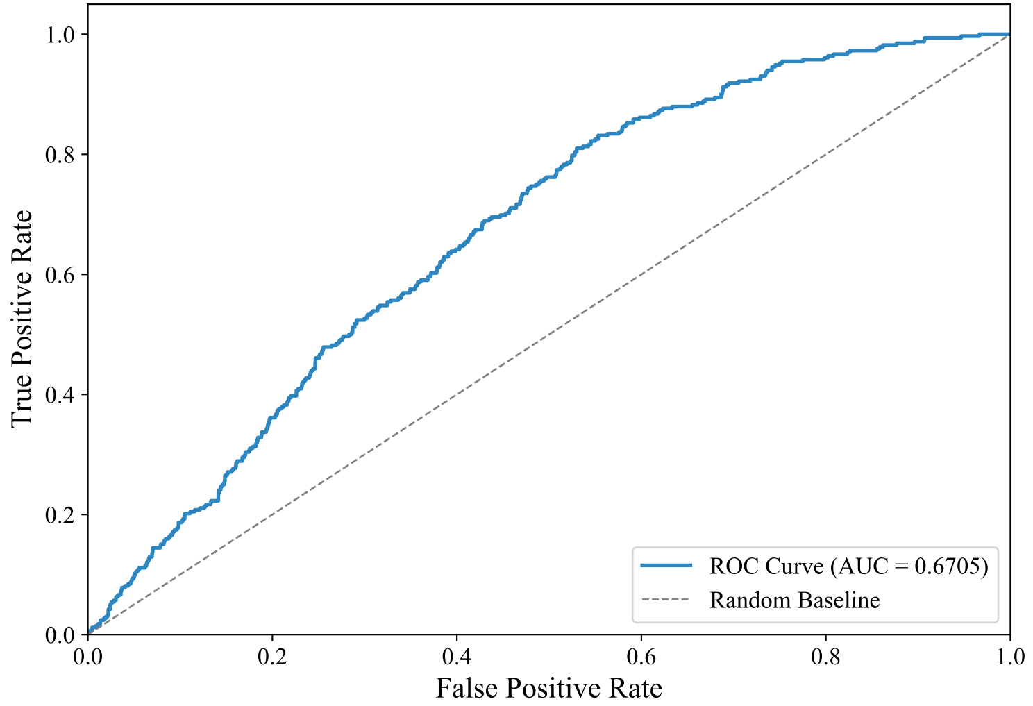
ROC Curve — GERMAN_MANUAL (paraphrase-multilingual-mpnet-base-v2, xgboost)
