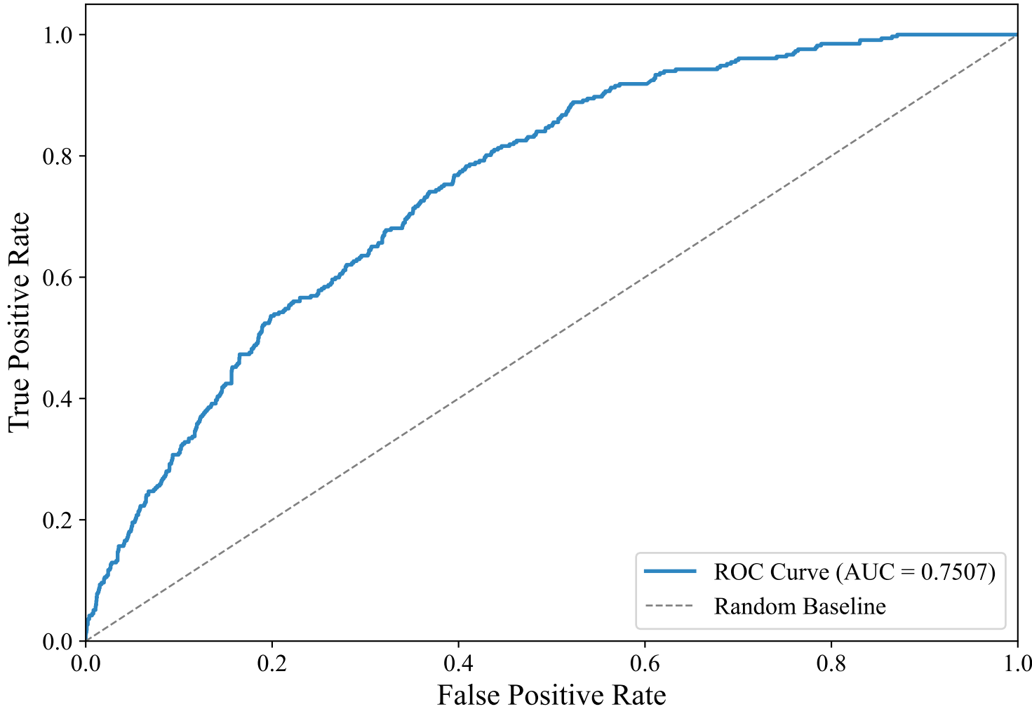
ROC Curve — GERMAN_MANUAL (snowflake-arctic-embed-l-v2.0, svm_rbf)
