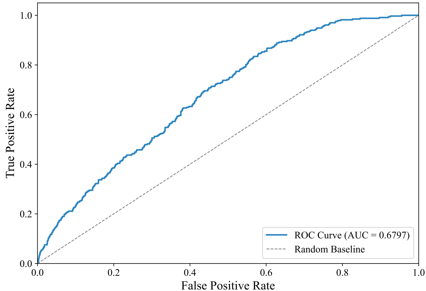
ROC Curve — GERMAN_MANUAL (xlm-roberta-base, svm_linear)
