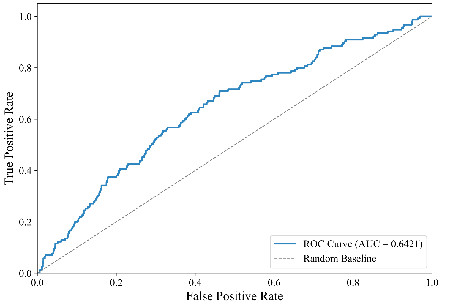
ROC Curve — SWEDISH_MANUAL (bert-base-multilingual-uncased, svm_linear)
