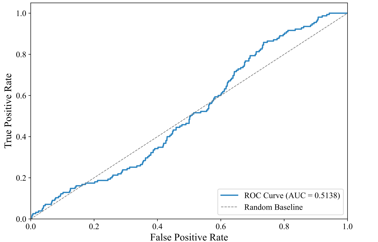
ROC Curve — SWEDISH_MANUAL (multilingual-e5-large-instruct, xgboost)
