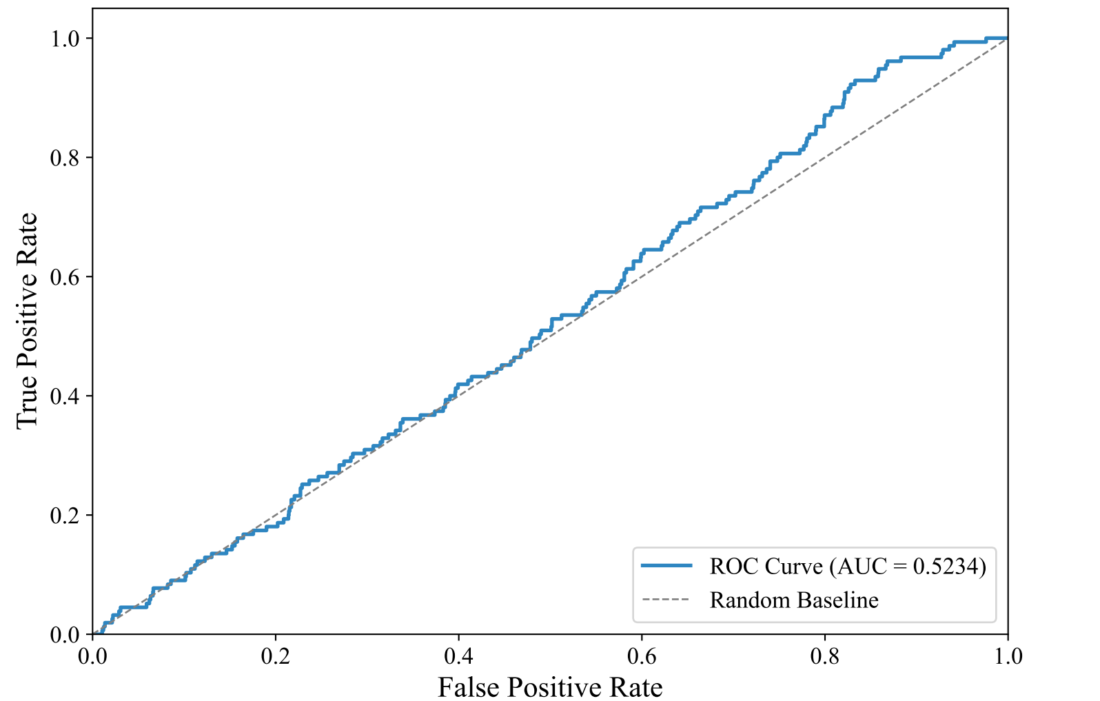
ROC Curve — SWEDISH_MANUAL (paraphrase-multilingual-MiniLM-L12-v2, random_forest)
