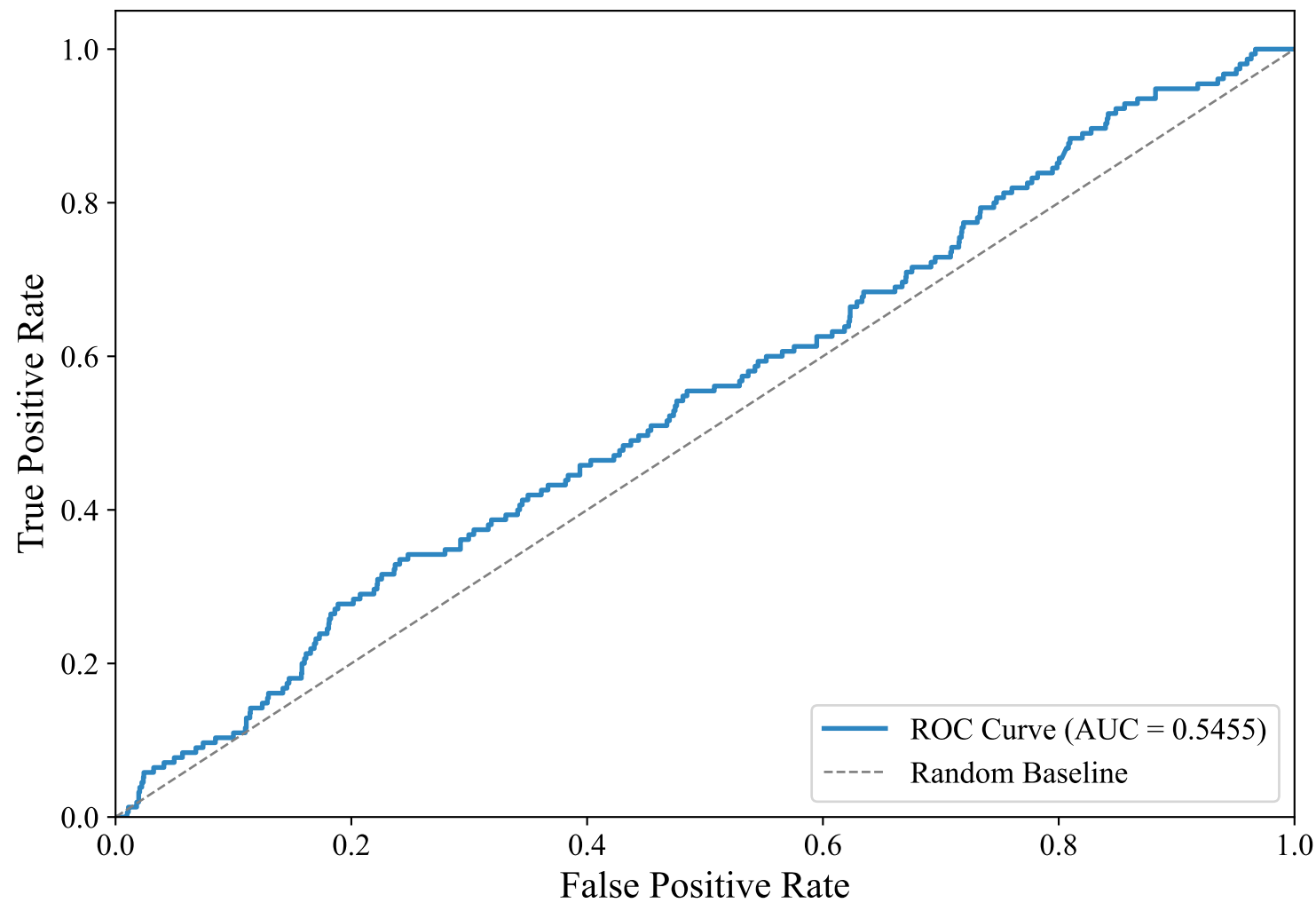
ROC Curve — SWEDISH_MANUAL (paraphrase-multilingual-MiniLM-L12-v2, svm_rbf)
