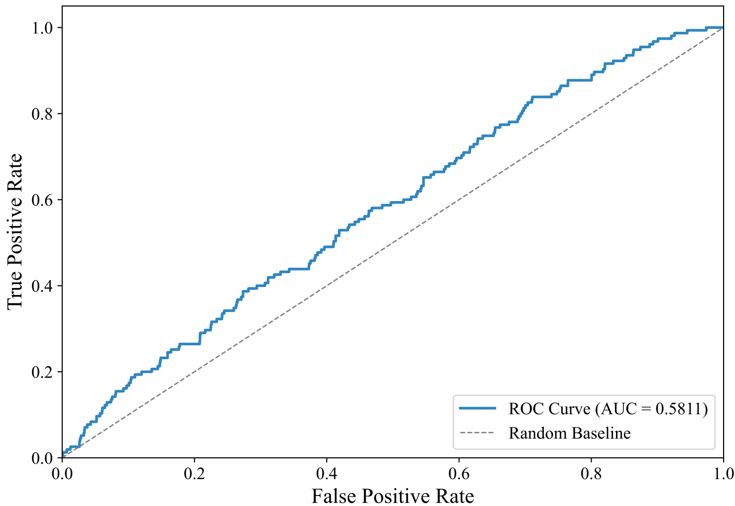
ROC Curve — SWEDISH_MANUAL (snowflake-arctic-embed-l-v2.0, svm_rbf)
