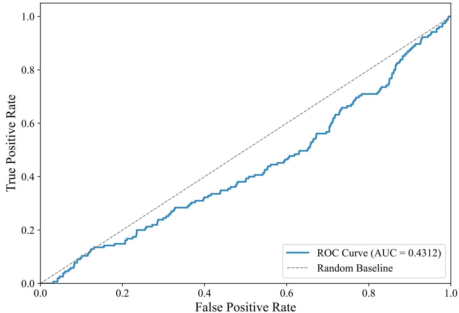
ROC Curve — SWEDISH_MANUAL (xlm-roberta-base, random_forest)
