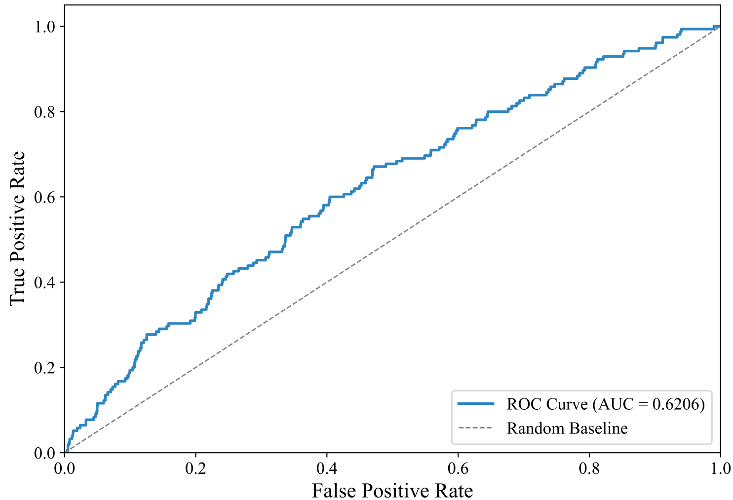
ROC Curve — SWEDISH_MANUAL (xlm-roberta-base, svm_linear)
