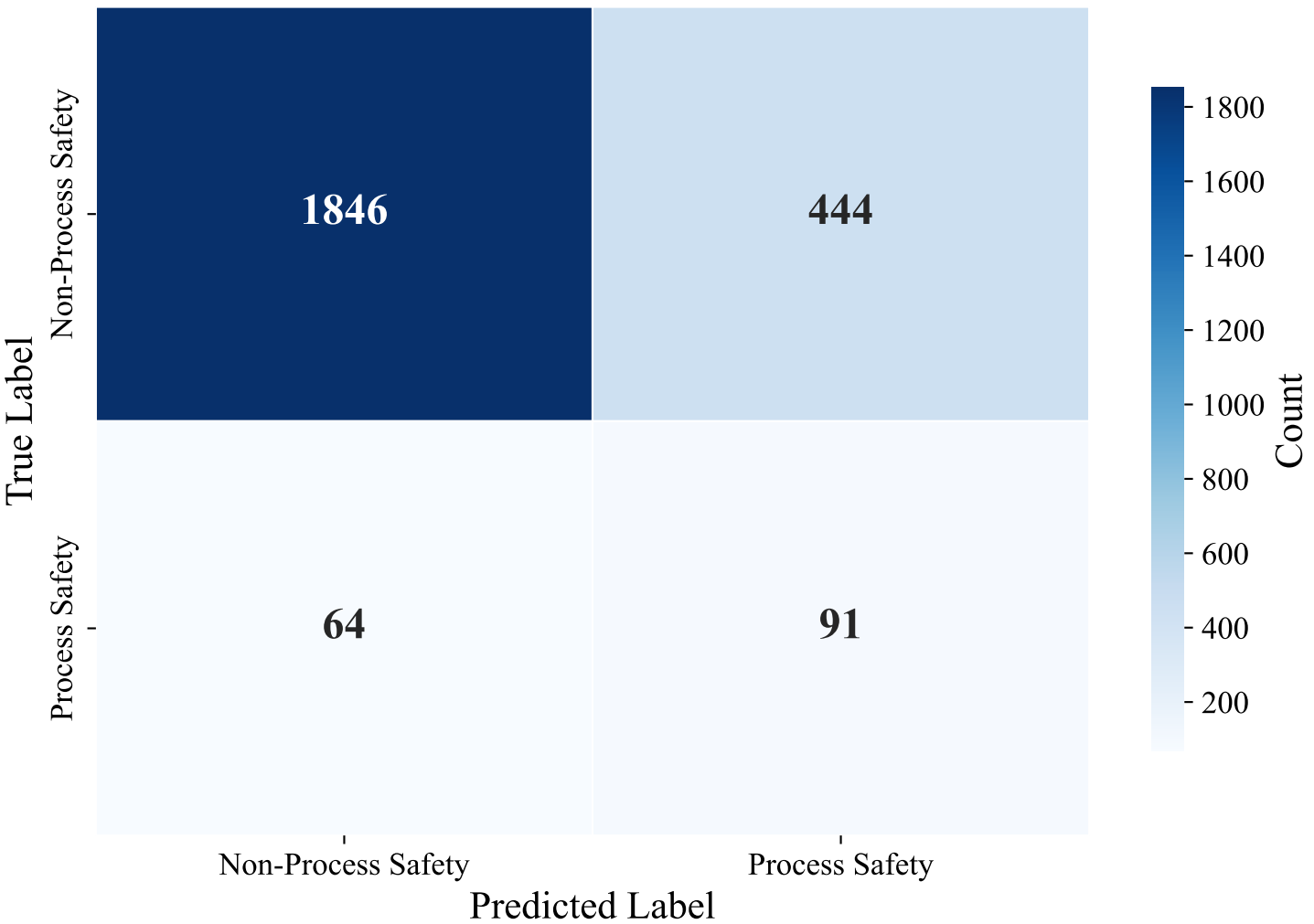
Confusion Matrix — SWEDEN (BERT-base-cased + LinearSVC)
