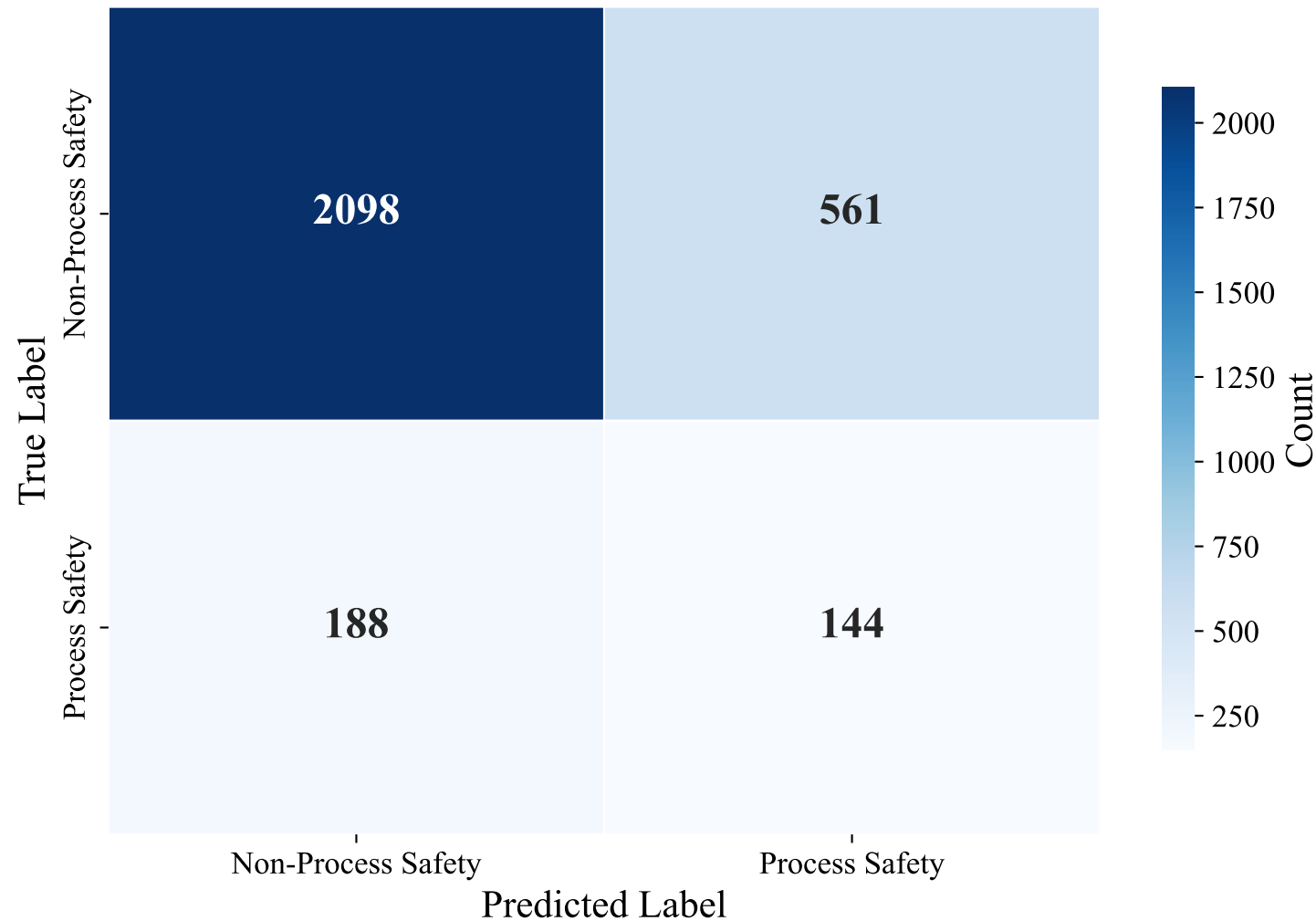
Confusion Matrix — GERMANY_MANUAL (xlnet-base-cased)
