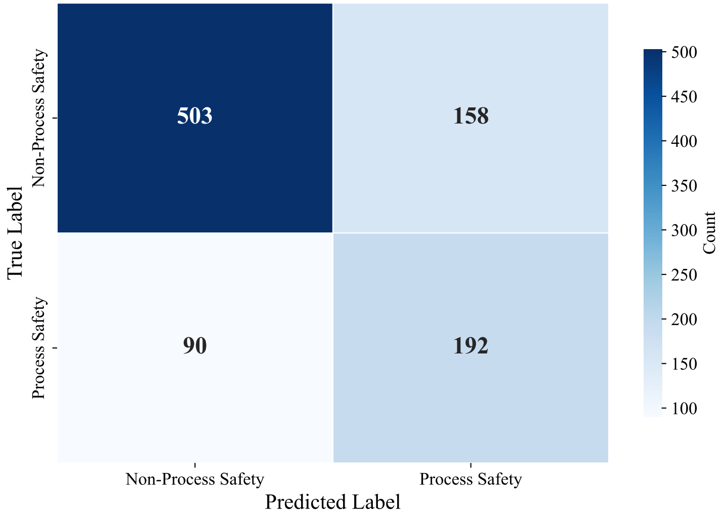
Confusion Matrix — ENGLISH_MANUAL (bert-base-multilingual-cased)
