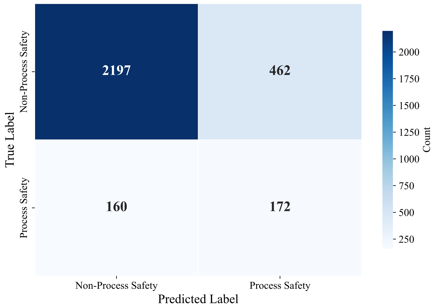
Confusion Matrix — GERMANY_MANUAL (bert-base-multilingual-uncased)
