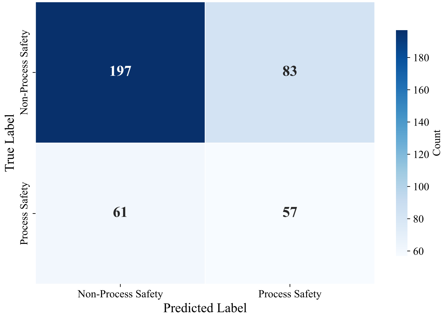
Confusion Matrix — NETHERLANDS_MANUAL (bert-base-multilingual-cased)
