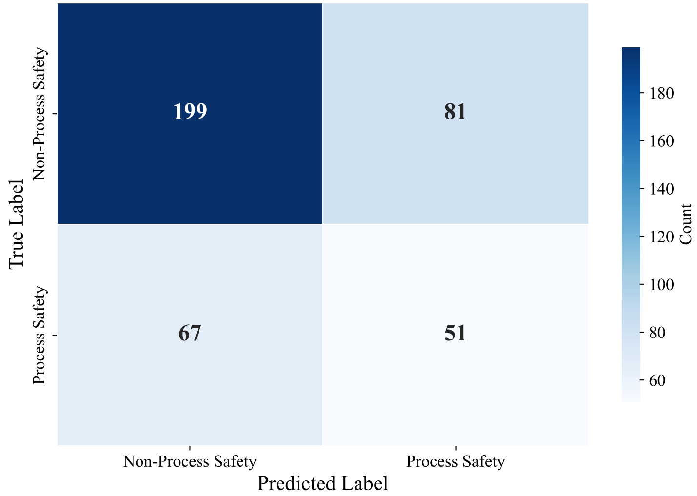
Confusion Matrix — NETHERLANDS_MANUAL (bert-base-multilingual-uncased)
