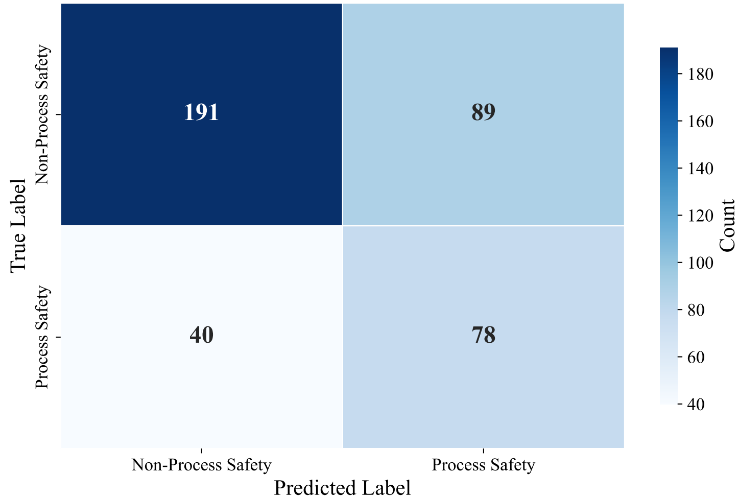
Confusion Matrix — DUTCH_MANUAL (paraphrase-multilingual-MiniLM-L12-v2, SVM)
