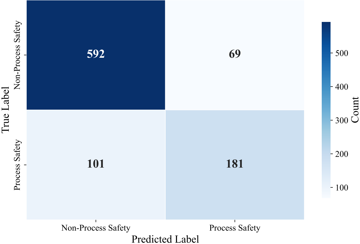
Confusion Matrix — ENGLISH MANUAL (paraphrase-multilingual-MiniLM-L12-v2, XGBoost)
