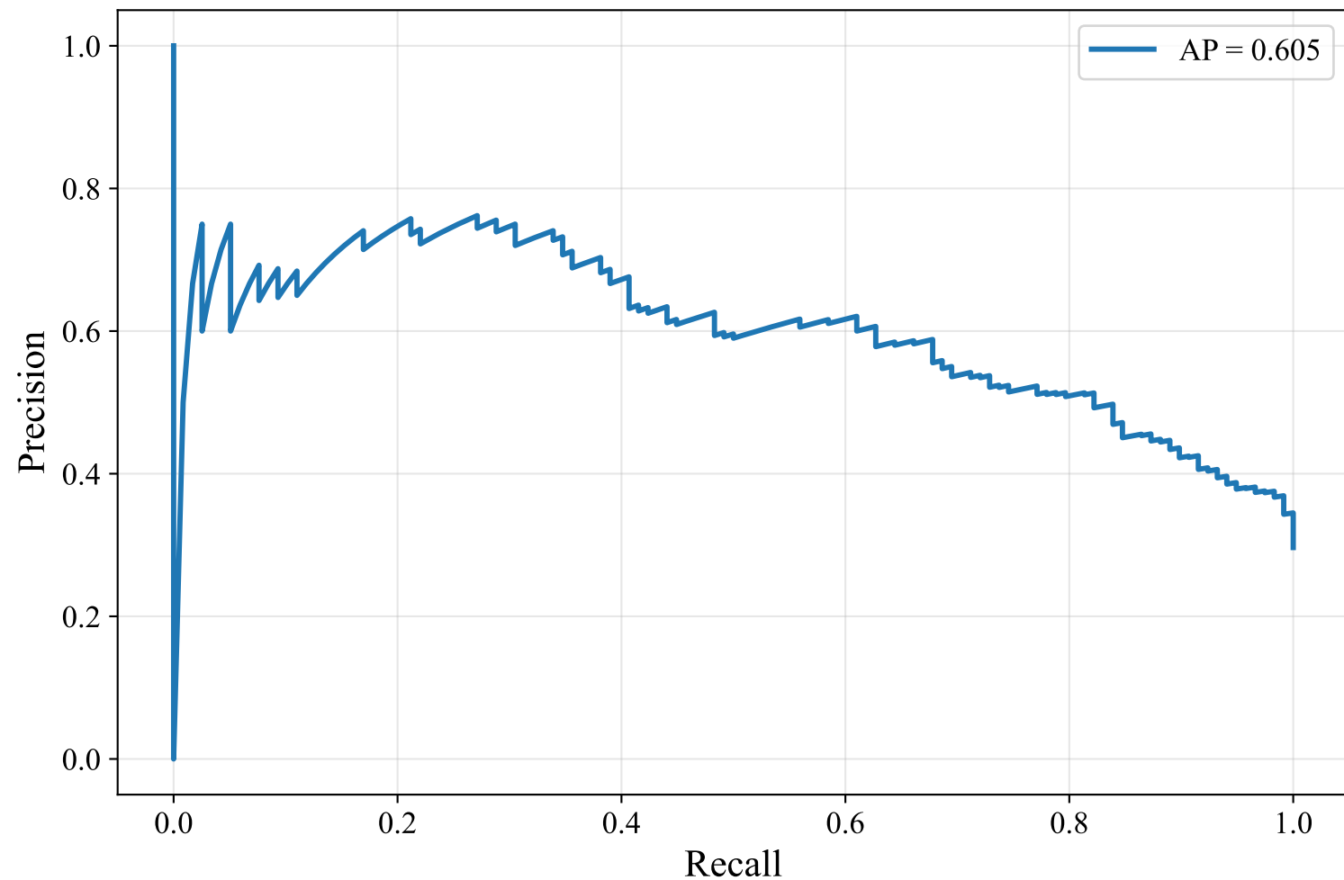
Precision-Recall Curve — DUTCH MANUAL (paraphrase-multilingual-MiniLM-L12-v2, XGBoost)
