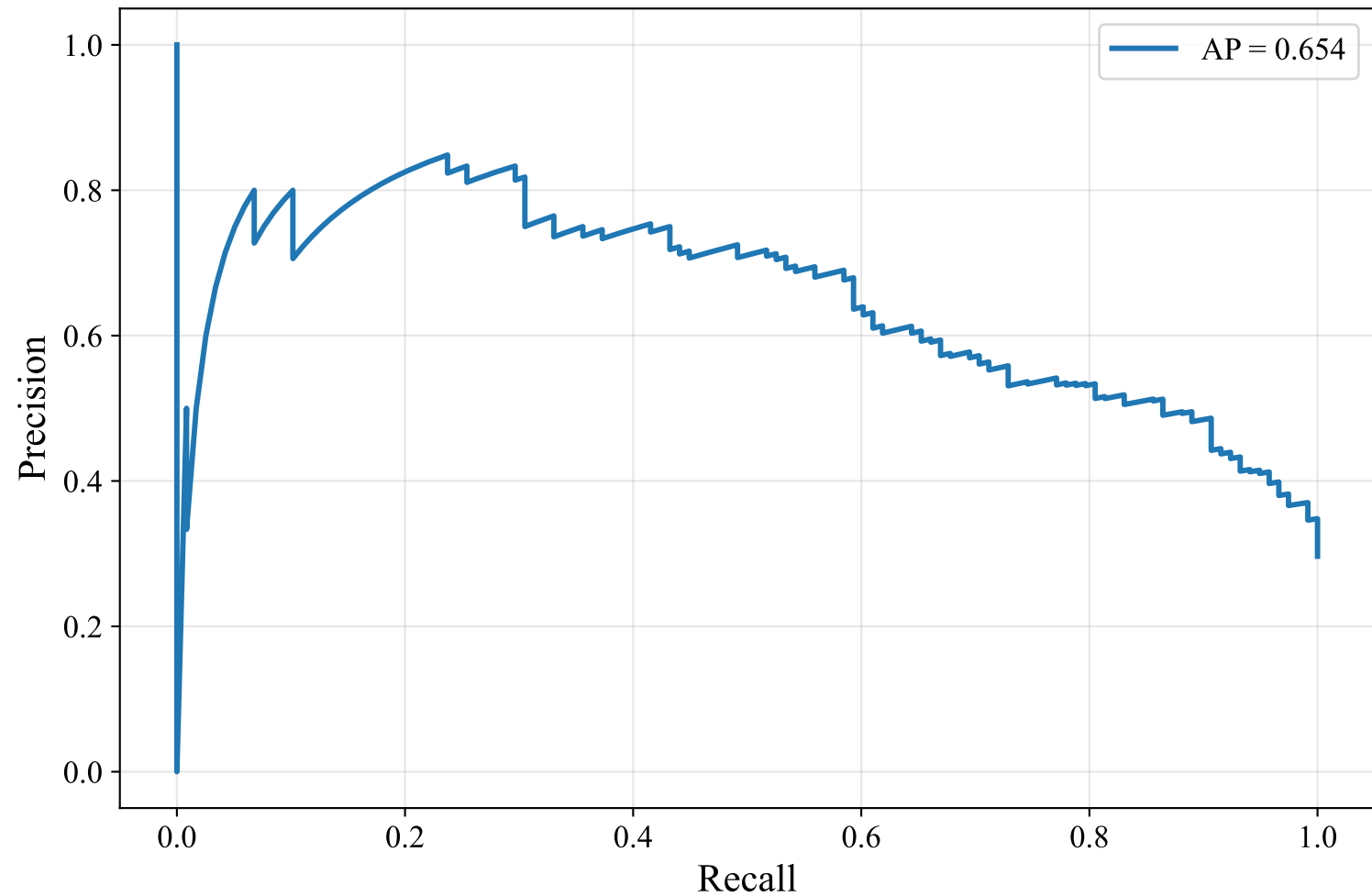
Precision-Recall Curve — DUTCH_MANUAL (snowflake-arctic-embed-l-v2.0, LightGBM)
