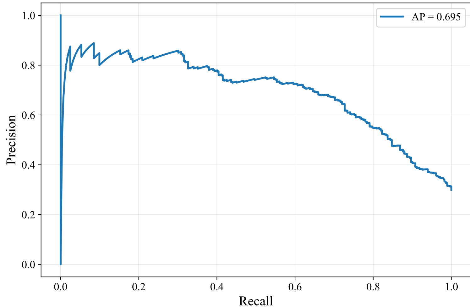
Precision-Recall Curve — ENGLISH_MANUAL (bert-base-multilingual-uncased, Random_Forest)
