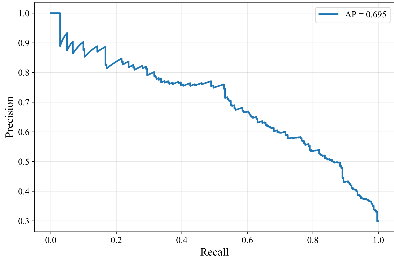
Precision-Recall Curve — ENGLISH_MANUAL (xlm-roberta-base, SVM)
