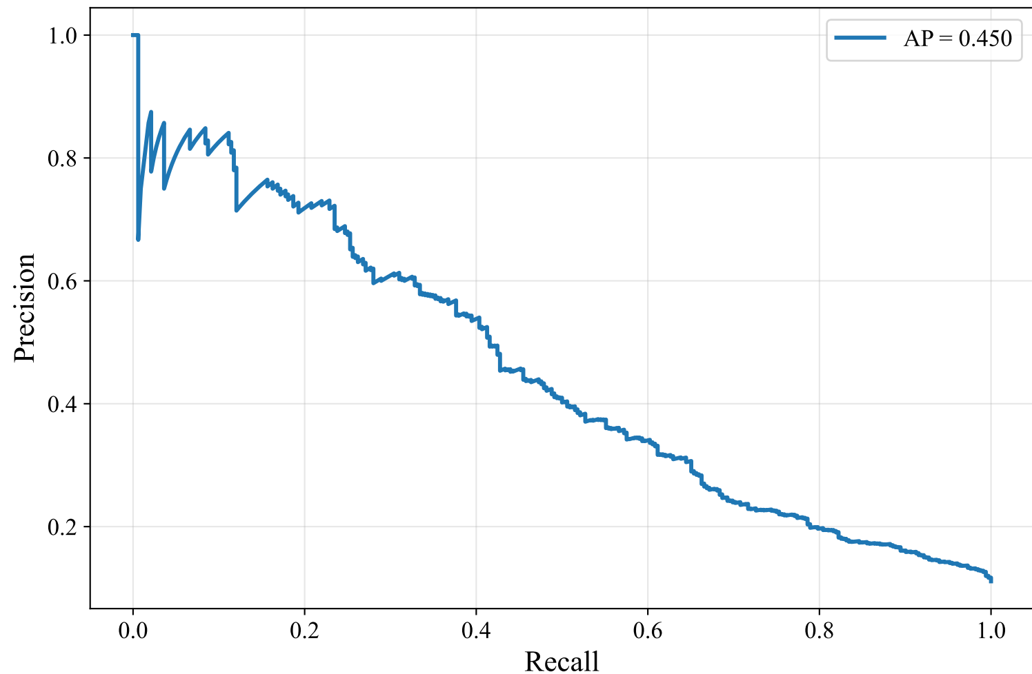
Precision-Recall Curve — GERMAN_MANUAL (paraphrase-multilingual-mpnet-base-v2, LightGBM)
