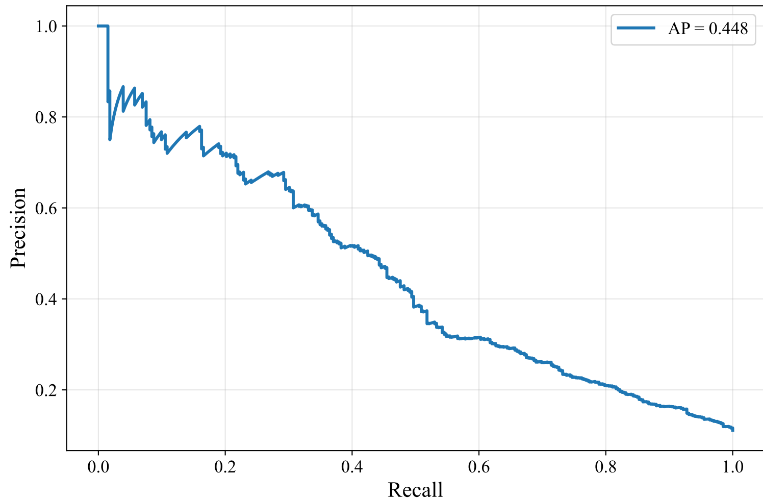
Precision-Recall Curve — GERMAN_MANUAL (paraphrase-multilingual-mpnet-base-v2, XGBoost)
