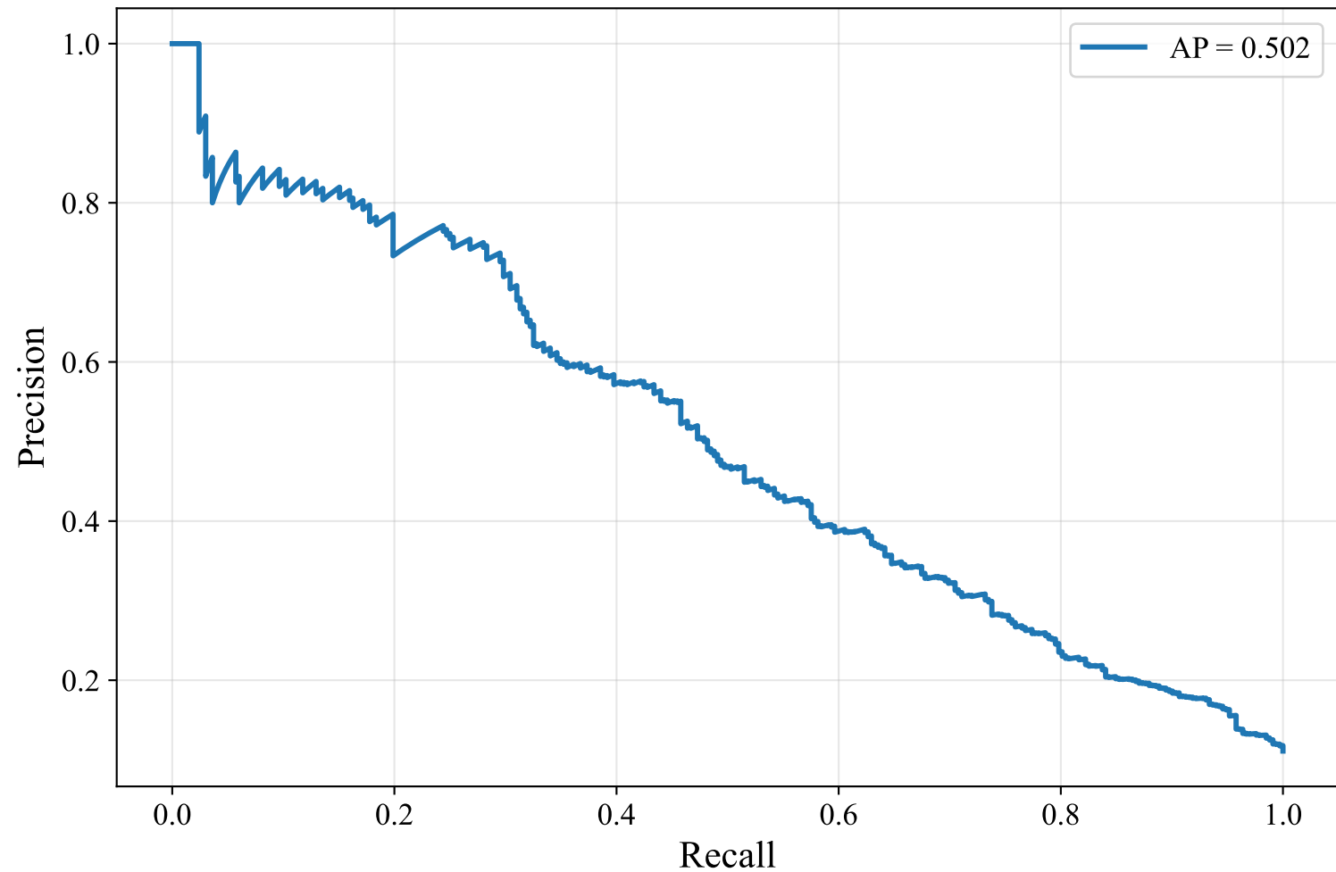
Precision-Recall Curve — GERMAN_MANUAL (snowflake-arctic-embed-l-v2.0, LightGBM)
