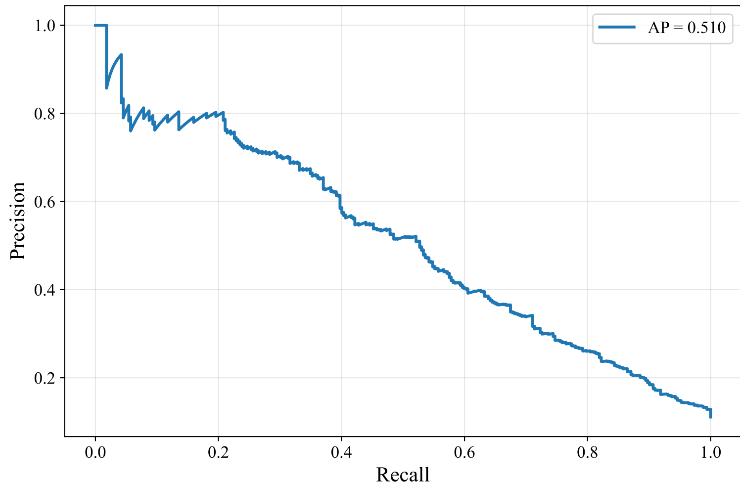
Precision-Recall Curve — GERMAN_MANUAL (snowflake-arctic-embed-l-v2.0, Random_Forest)
