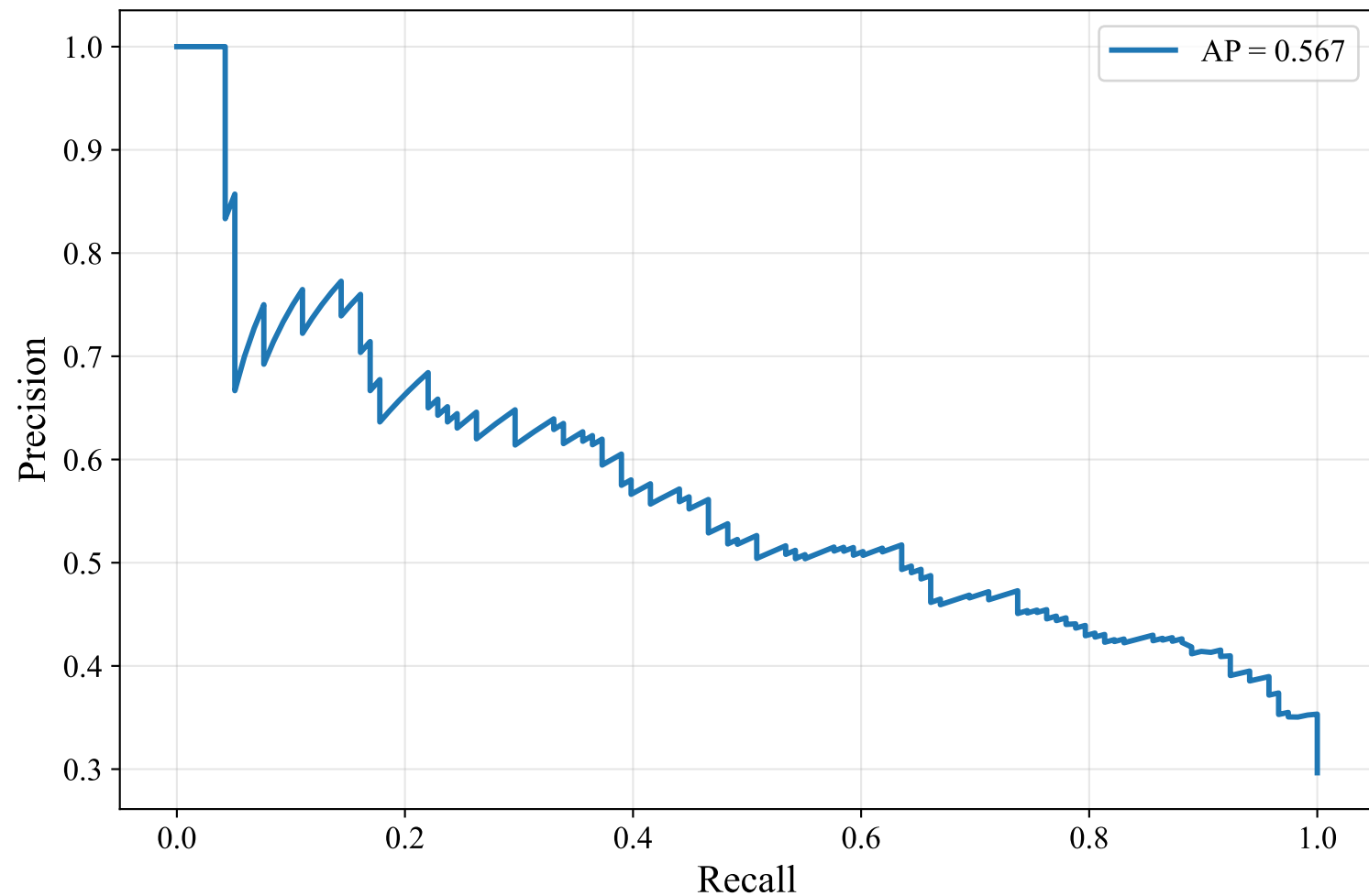
Precision-Recall Curve — NETHERLANDS_MANUAL (bert-base-multilingual-uncased, Random_Forest)
