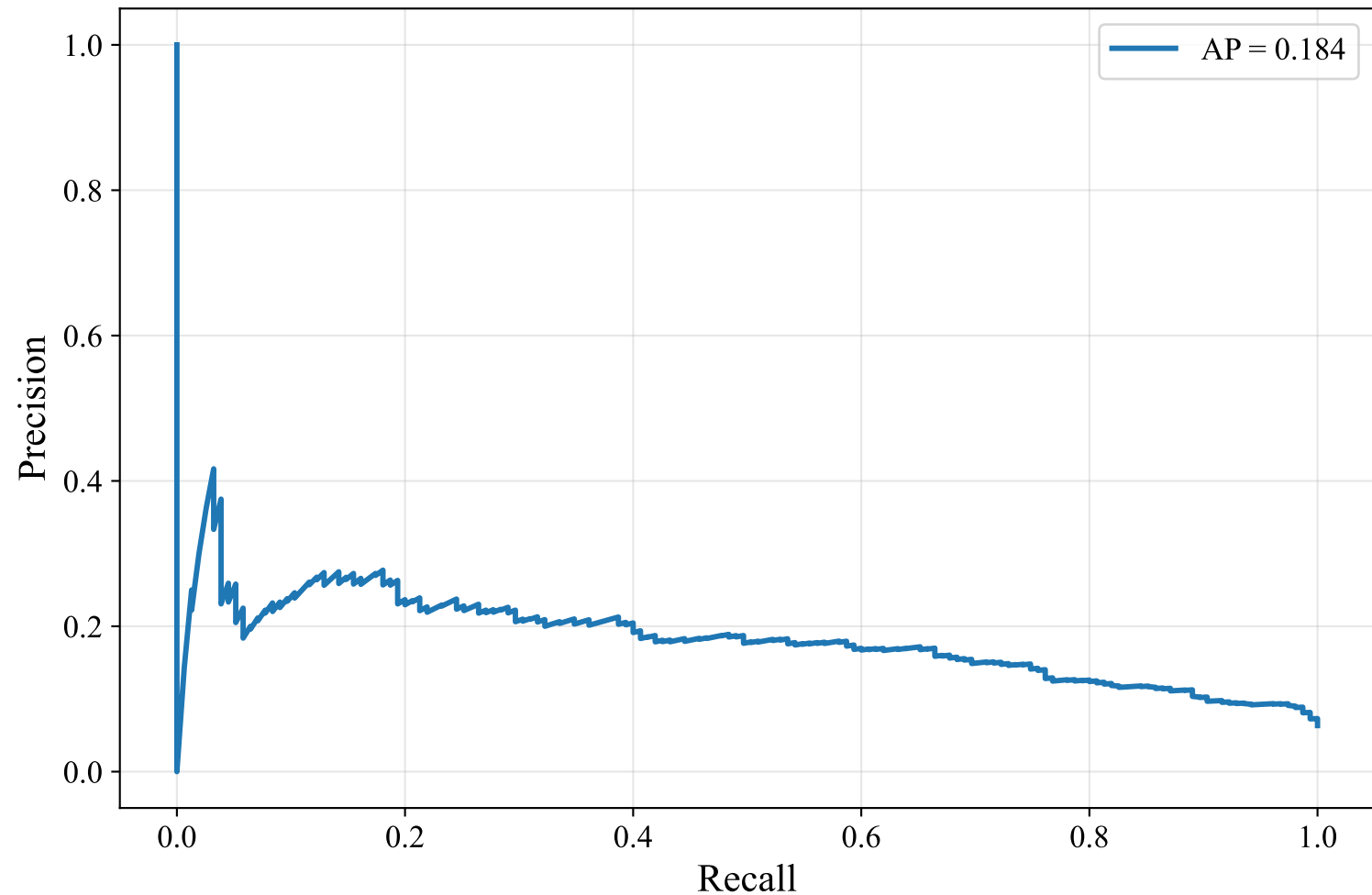
Precision-Recall Curve — SWEDISH_MANUAL (paraphrase-multilingual-MiniLM-L12-v2, Random_Forest)
