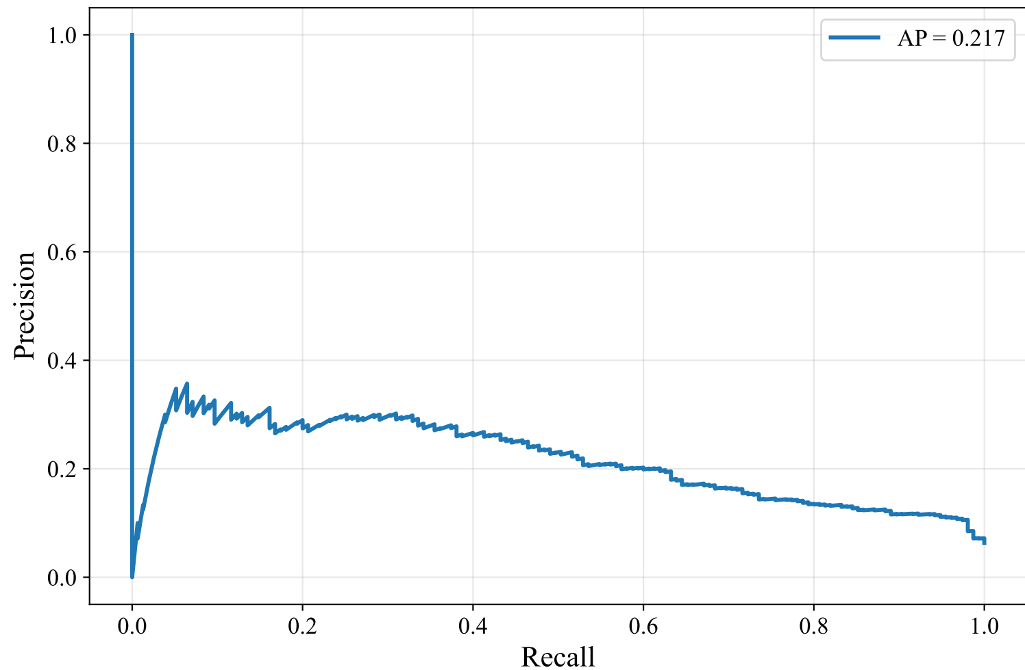
Precision-Recall Curve — SWEDISH_MANUAL (snowflake-arctic-embed-l-v2.0, Random_Forest)
