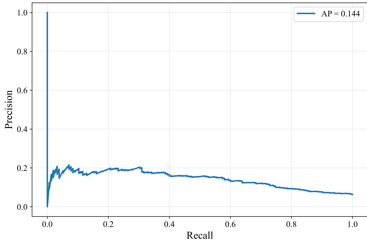
Precision-Recall Curve — SWEDISH_MANUAL (xlm-roberta-base, SVM)
