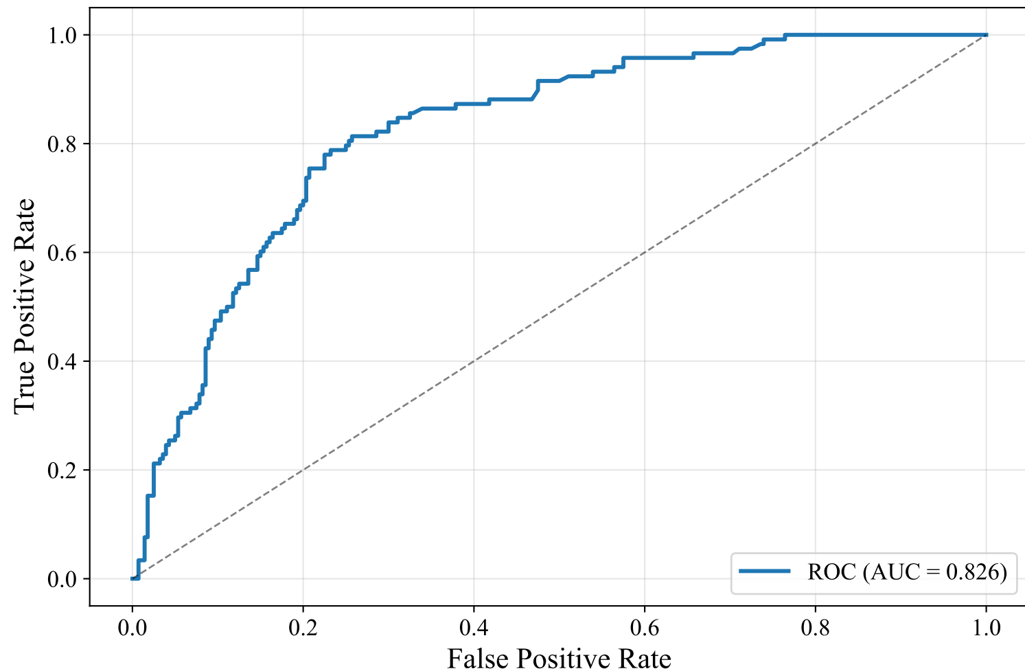
ROC Curve — DUTCH_MANUAL (paraphrase-multilingual-mpnet-base-v2, Random_Forest)
