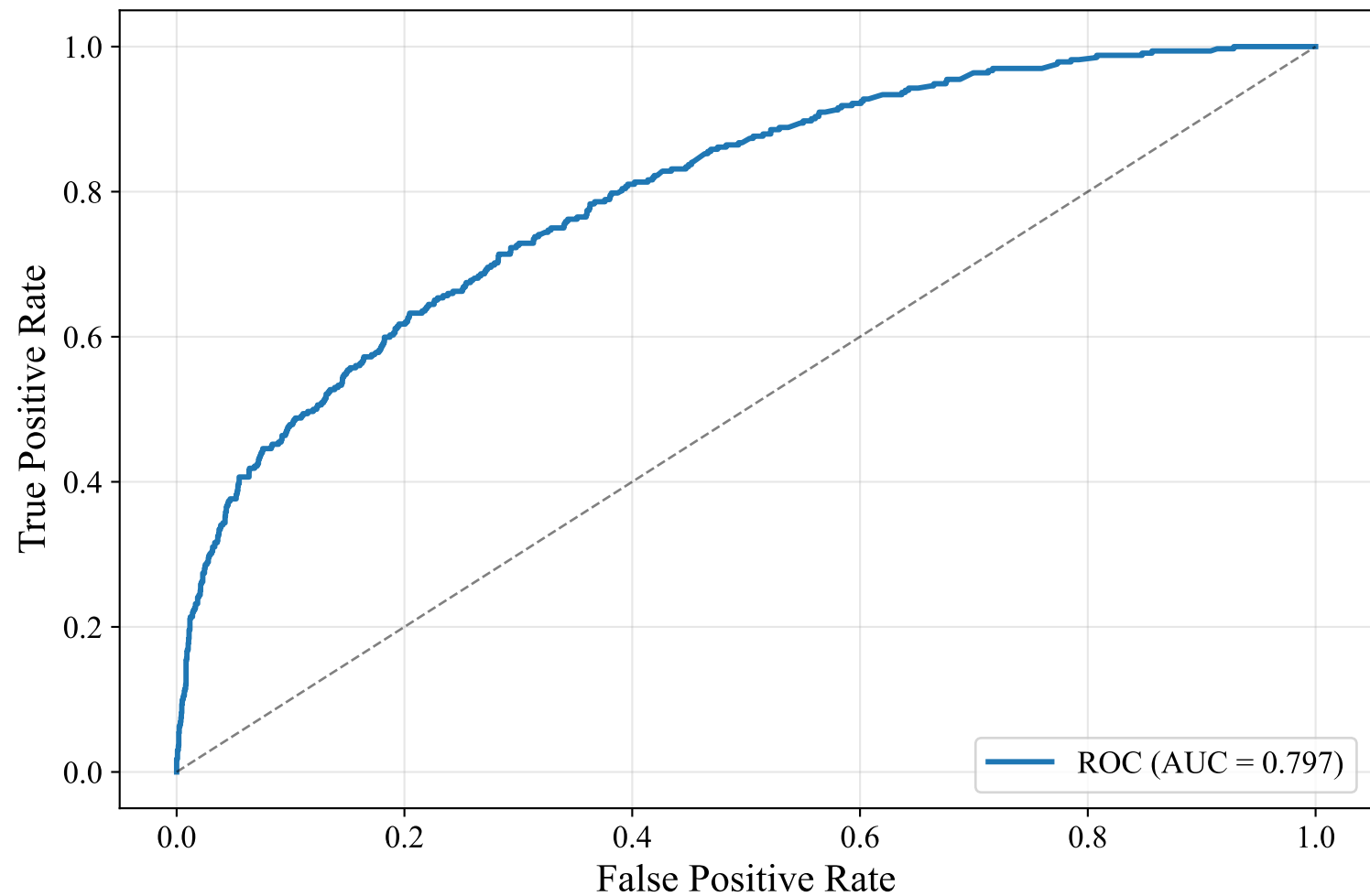
ROC Curve — GERMAN_MANUAL (paraphrase-multilingual-mpnet-base-v2, Random_Forest)
