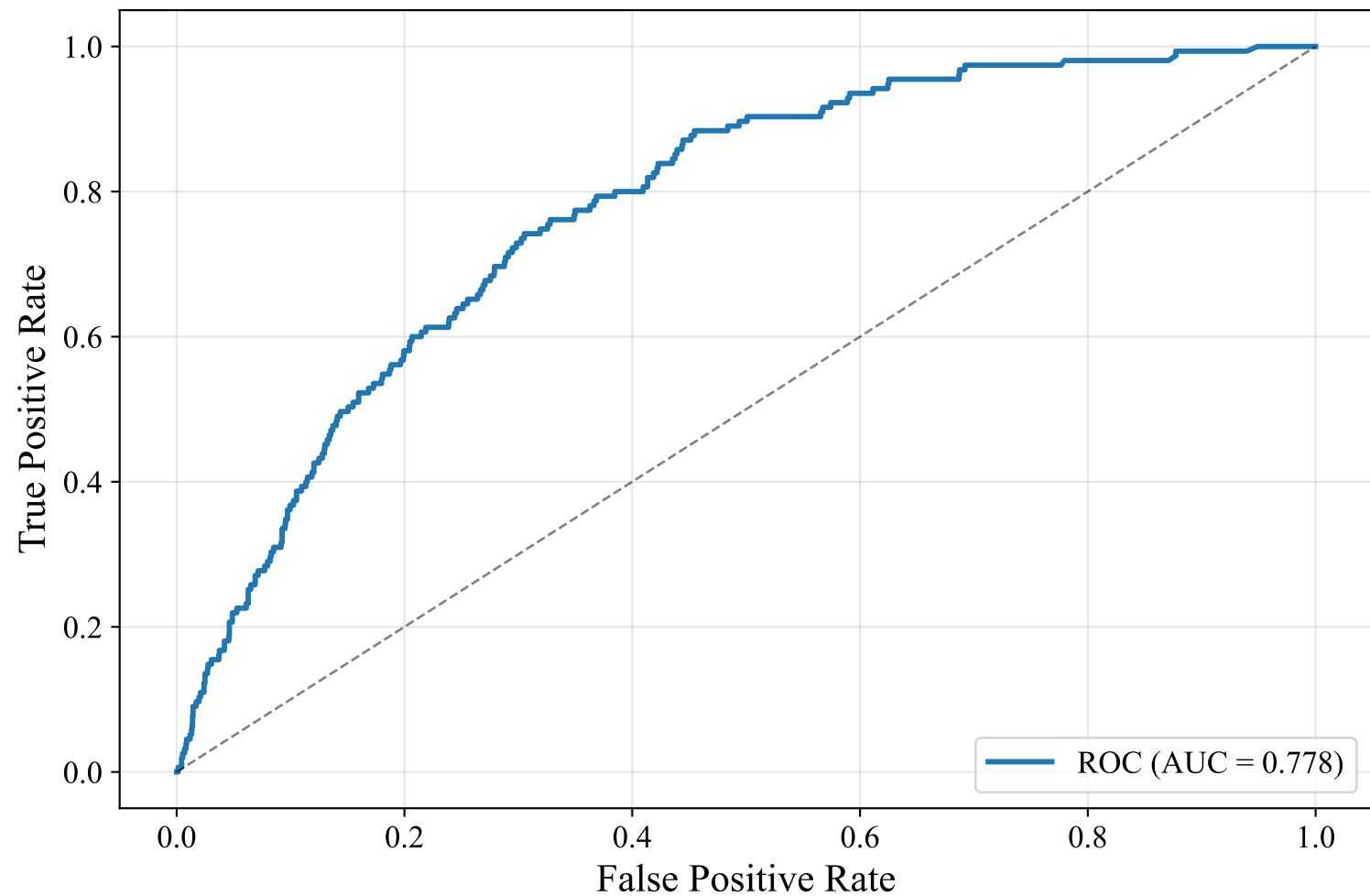
ROC Curve — SWEDEN_MANUAL (bert-base-multilingual-uncased, Random_Forest)
