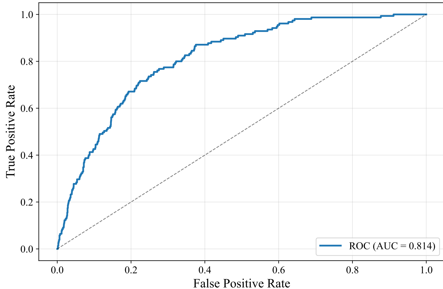
ROC Curve — SWEDISH_MANUAL (snowflake-arctic-embed-l-v2.0, LightGBM)
