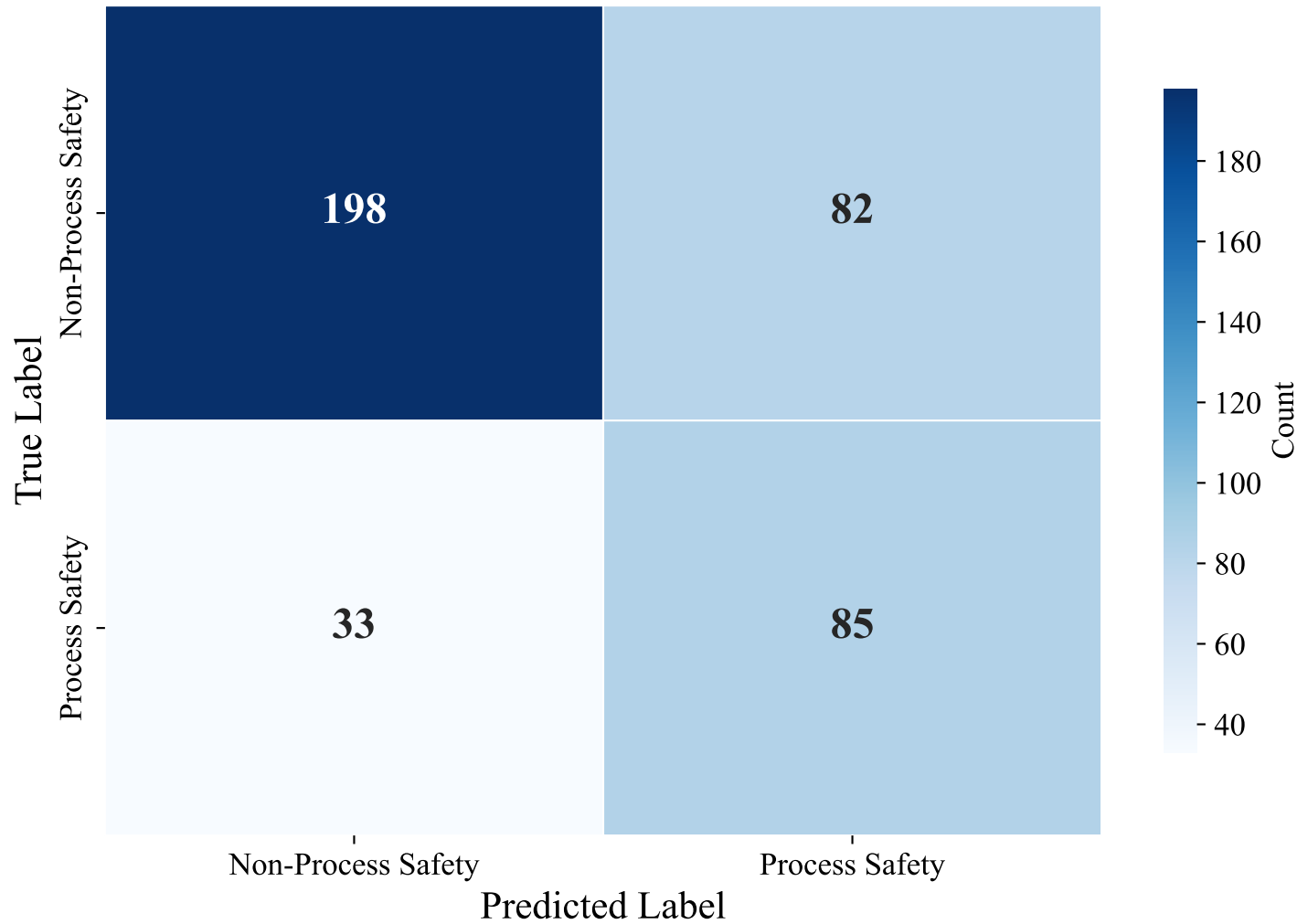
Confusion Matrix — DUTCH_MANUAL (paraphrase-multilingual-MiniLM-L12-v2, XGBoost)
