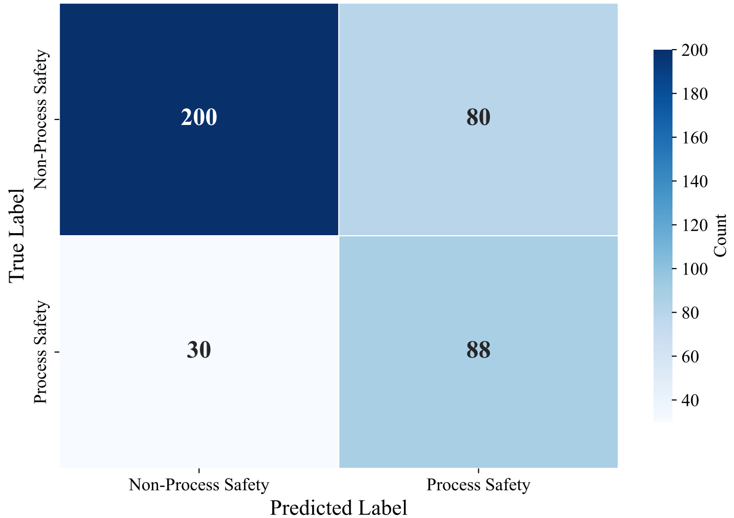
Confusion Matrix — DUTCH_MANUAL (paraphrase-multilingual-mpnet-base-v2, XGBoost_Optimized)
