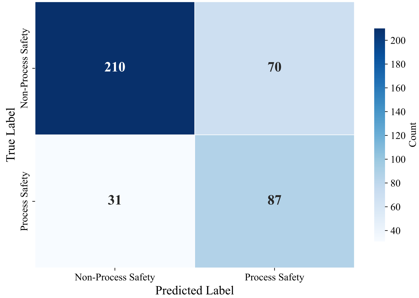
Confusion Matrix — DUTCH_MANUAL (snowflake-arctic-embed-l-v2.0, LightGBM_Optimized)
