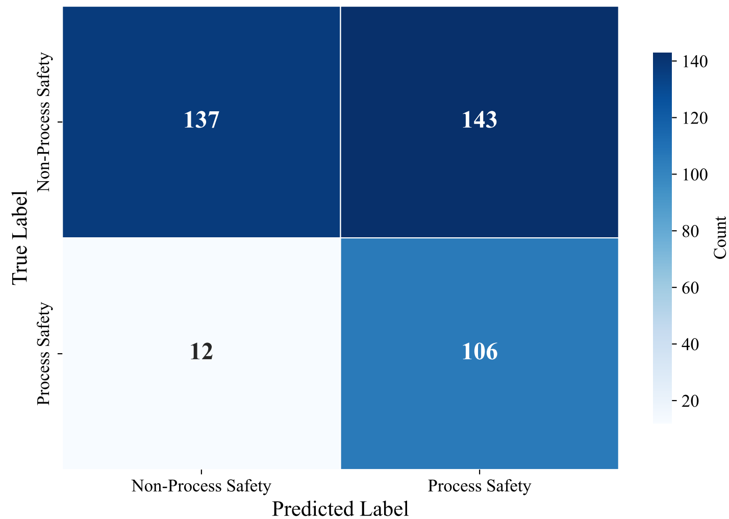
Confusion Matrix — DUTCH_MANUAL (snowflake-arctic-embed-l-v2.0, Random_Forest)
