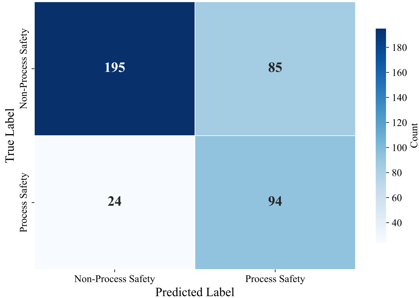
Confusion Matrix — DUTCH_MANUAL (snowflake-arctic-embed-l-v2.0, XGBoost_Optimized)
