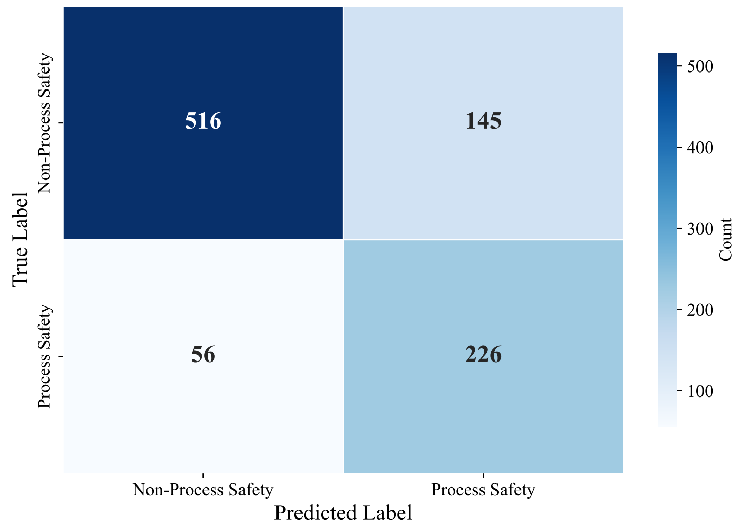
Confusion Matrix — ENGLISH_MANUAL (paraphrase-multilingual-MiniLM-L12-v2, LightGBM)
