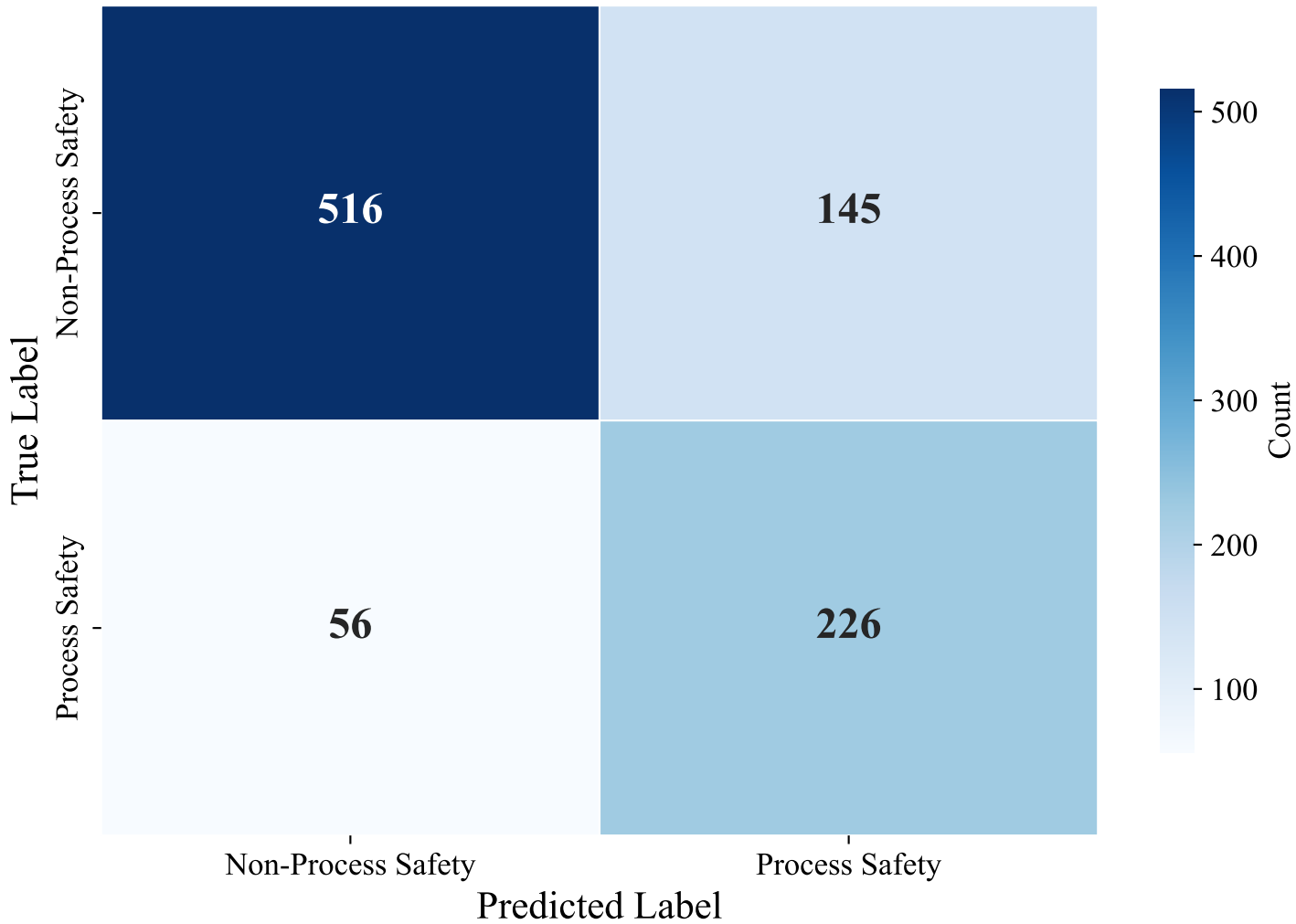
Confusion Matrix — ENGLISH_MANUAL (paraphrase-multilingual-MiniLM-L12-v2, LightGBM_Optimized)
