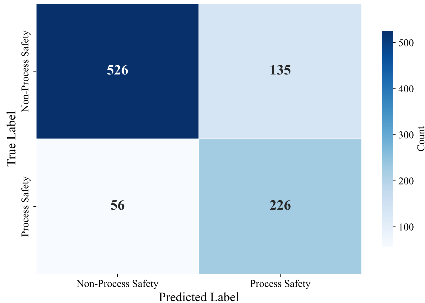
Confusion Matrix — ENGLISH_MANUAL (snowflake-arctic-embed-l-v2.0, LightGBM)
