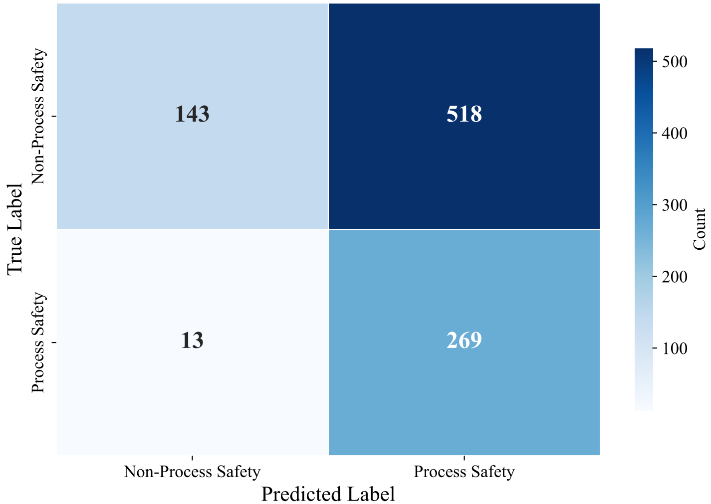
Confusion Matrix — ENGLISH_MANUAL (snowflake-arctic-embed-l-v2.0, Random_Forest_Optimized)
