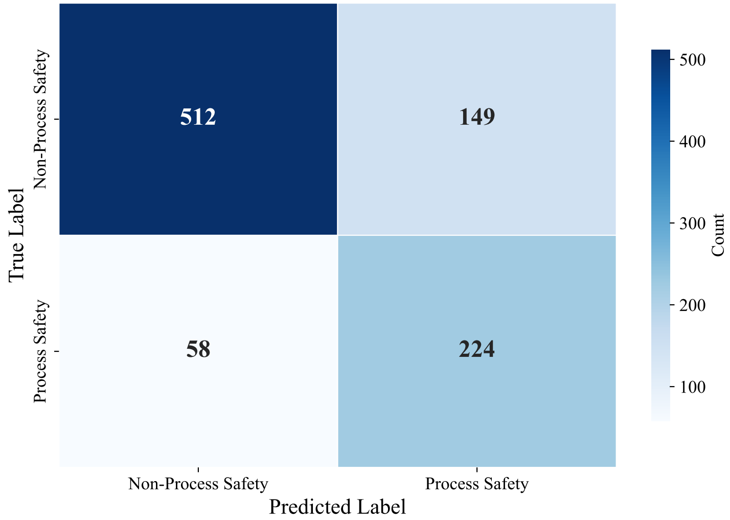
Confusion Matrix — ENGLISH_MANUAL (snowflake-arctic-embed-l-v2.0, XGBoost)
